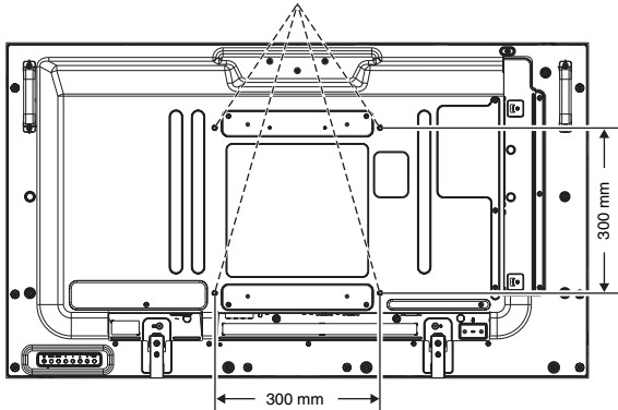
VESA-Montageadapter
